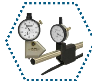
INTERNAL & EXTERNAL THREAD HEIGHT GAGE
