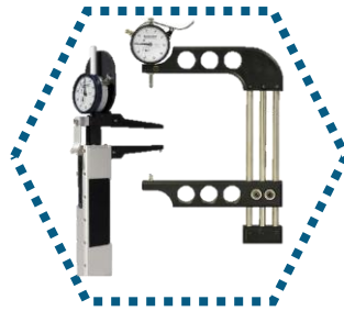
INTERNAL & EXTERNAL TAPER GAGE
